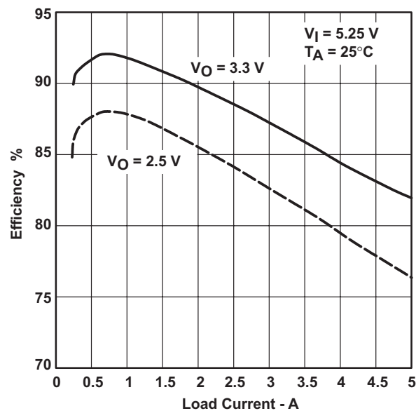
Figure 26. Converter Efficiency
